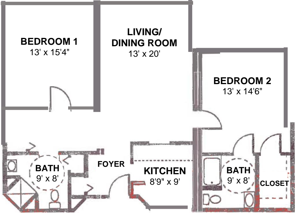
Floor Plan A—1,170 sq.ft.
